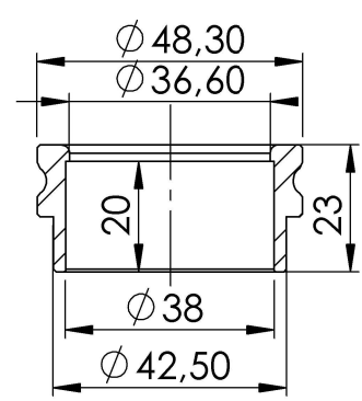
4 S.S. Cilinder bushing Cod.206432
