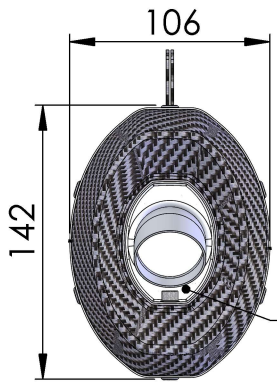
Factory S silencer Carbon Øi 60 RHS Cod.308471481
